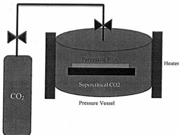
Figure 1: Schematic diagram illustrating supercritical fluid pressure vessel for perovskite film processing.
